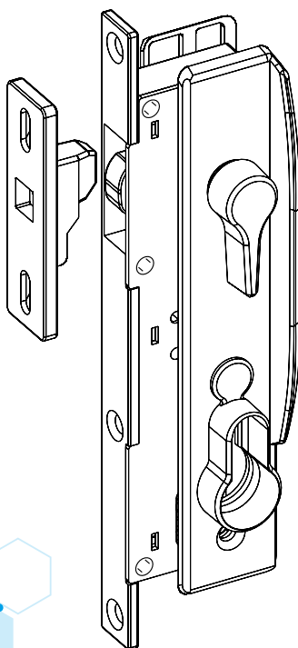
Lockset with square handle set
